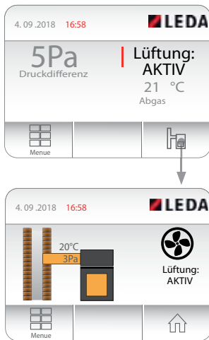
Abb. 5.5 System-Ebene
